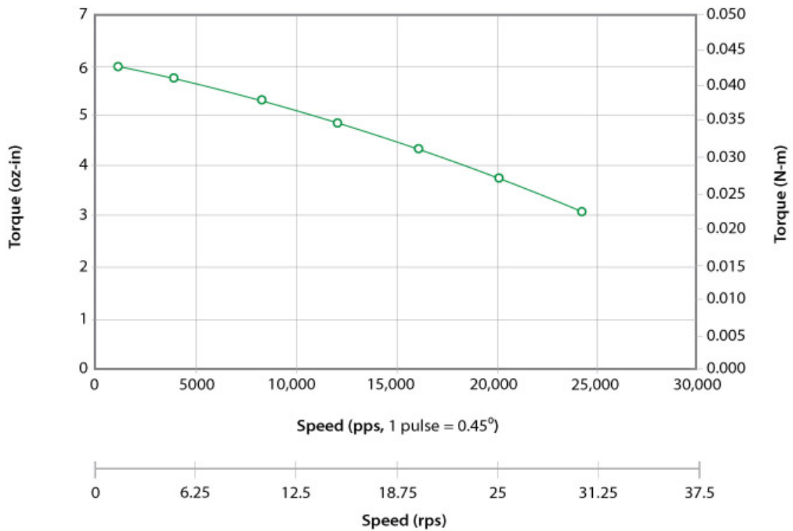
4109X-51 24VDC, 0.6 Amps/Phase, Bipolar, 1/2 Stepping
